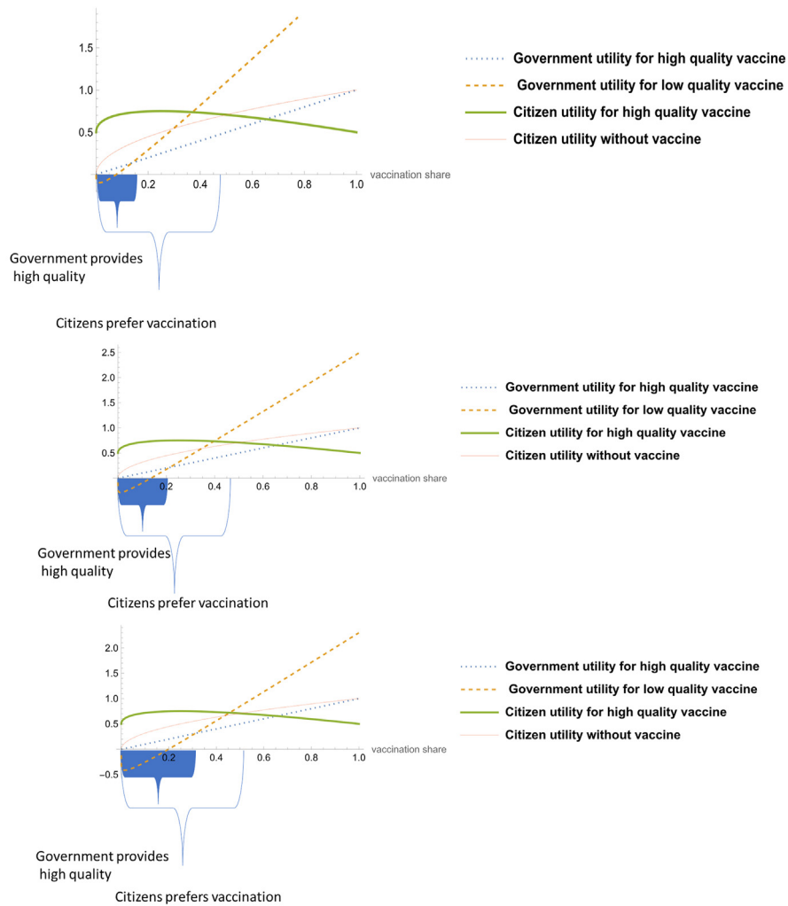
Note: The figures are for \alpha = 0.3, \gamma = 0.5, \alpha = 0.1, \gamma = 0.5 and \alpha = 0.1, \gamma = 0.7 , respectively.
